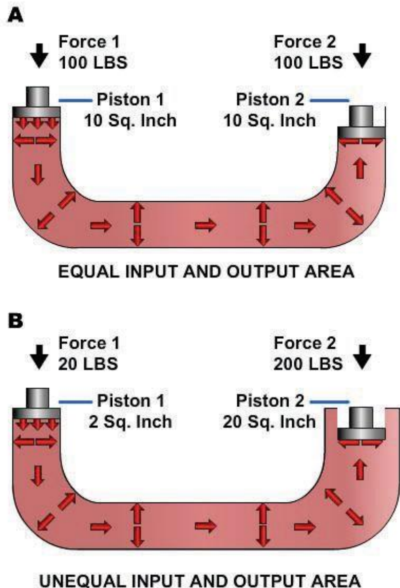
Figure 2-14 — Principle of mechanical hydraulics.
