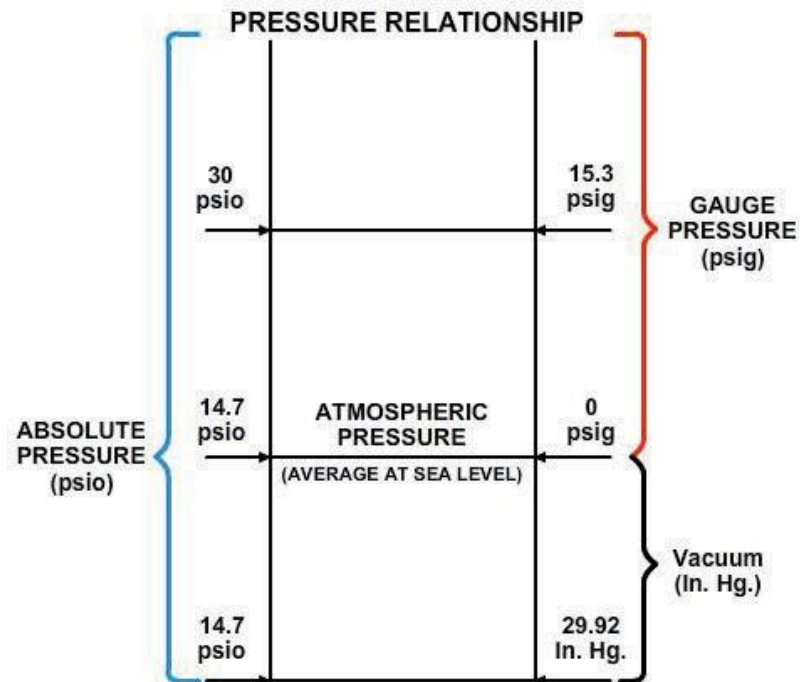
Figure 2-11 — Relationships among gauge pressure, atmospheric pressure, vacuum, and absolute pressure.
