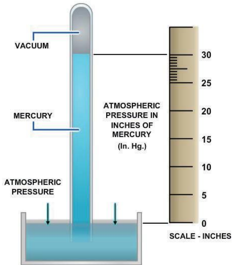
Figure 2-12 — Typical barometer.
