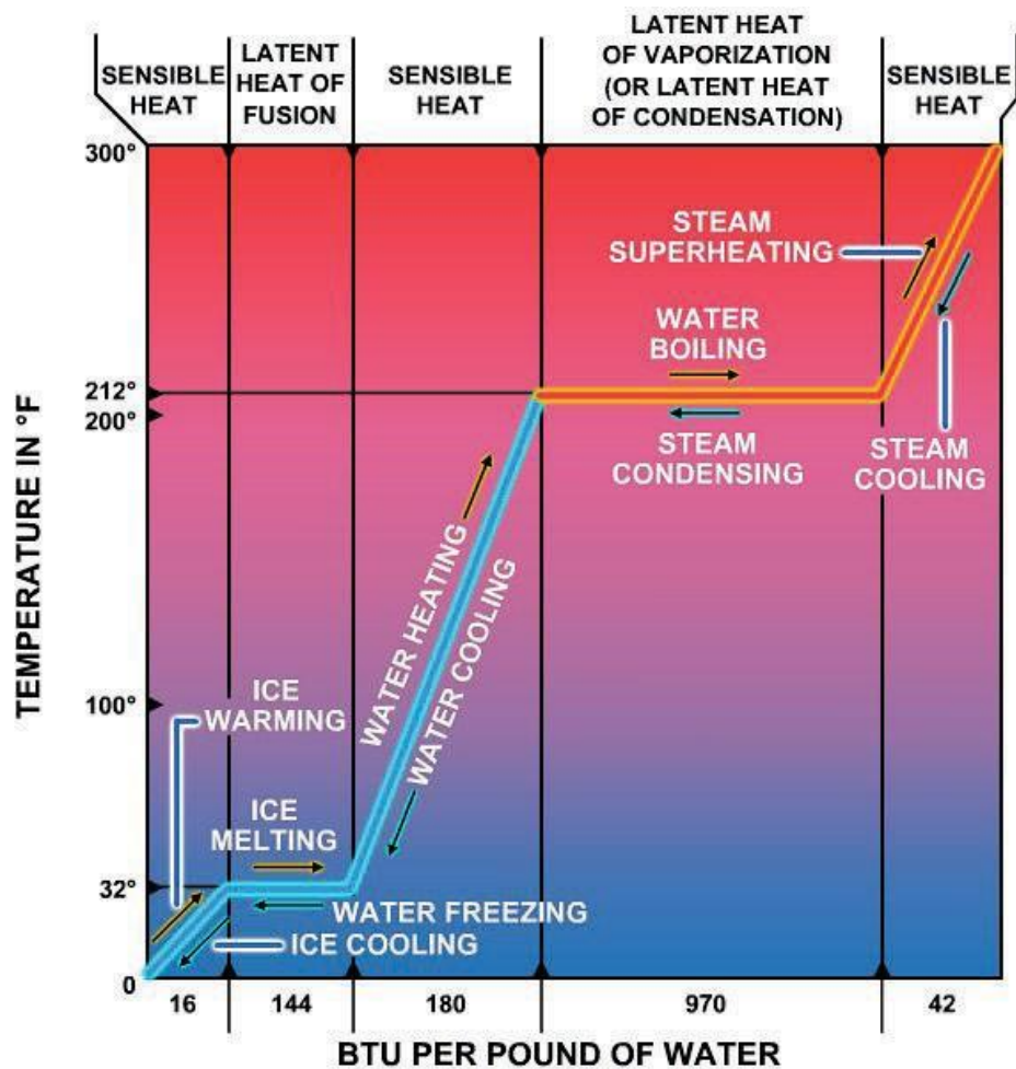
Figure 2-9 — Relationship between sensible heat and latent heat.
