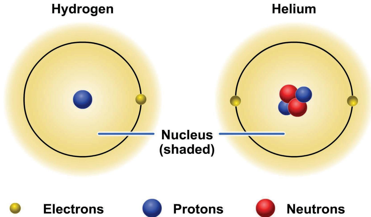
Figure 2-1 — Structure of simple atoms.
