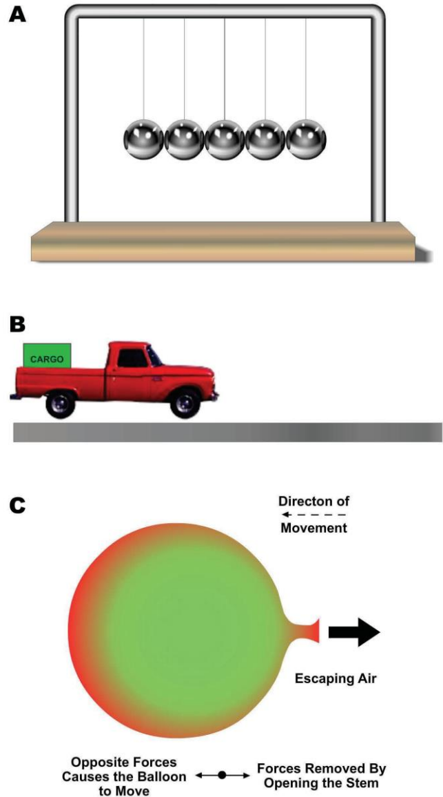
Figure 2-4 — Newton's three laws.
