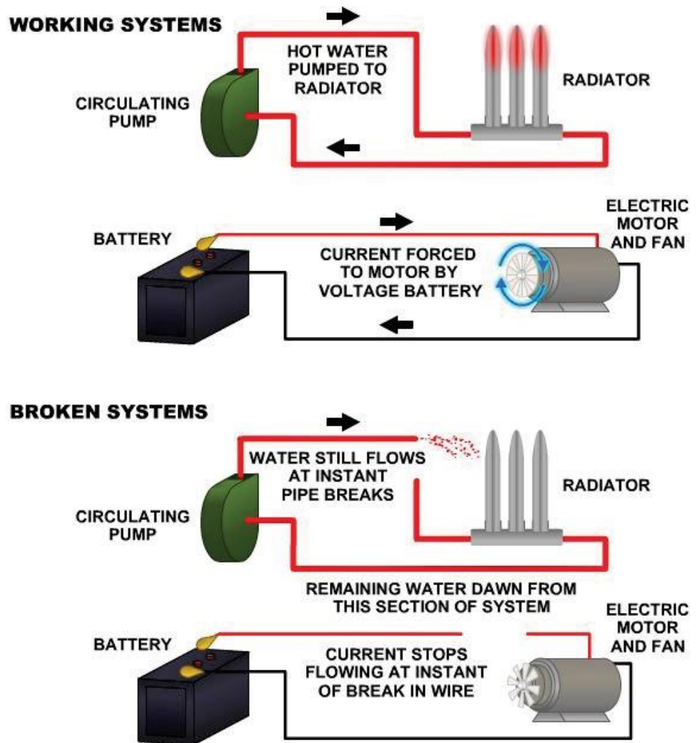
Figure 2-3 — Different characteristics of current and water.
